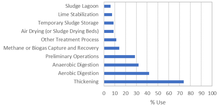
Biosolids Treatment Processes
