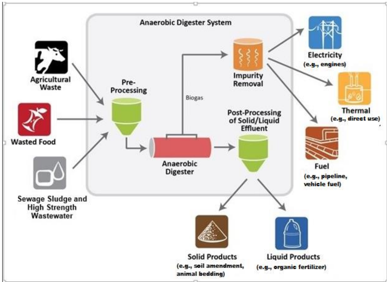
Figure 1. Anaerobic System Components
