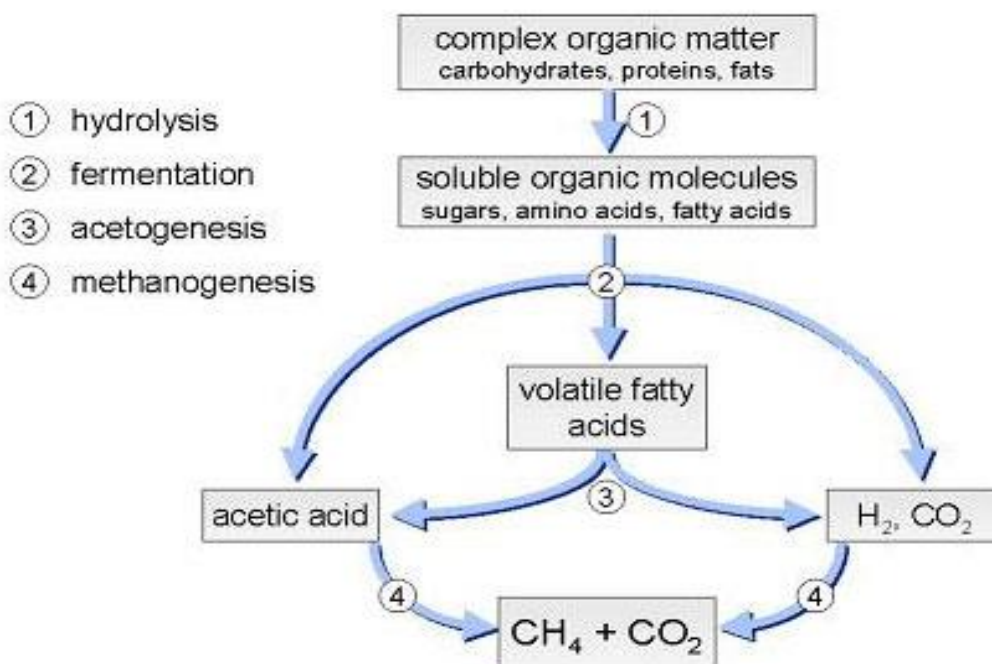
Figure 2. The chemical reactions that occur during anaerobic digestion
