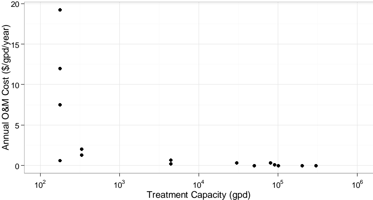
Figure IV-18. Annual O&M costs and treatment capacities for decentralized treatment systems (2012$).
