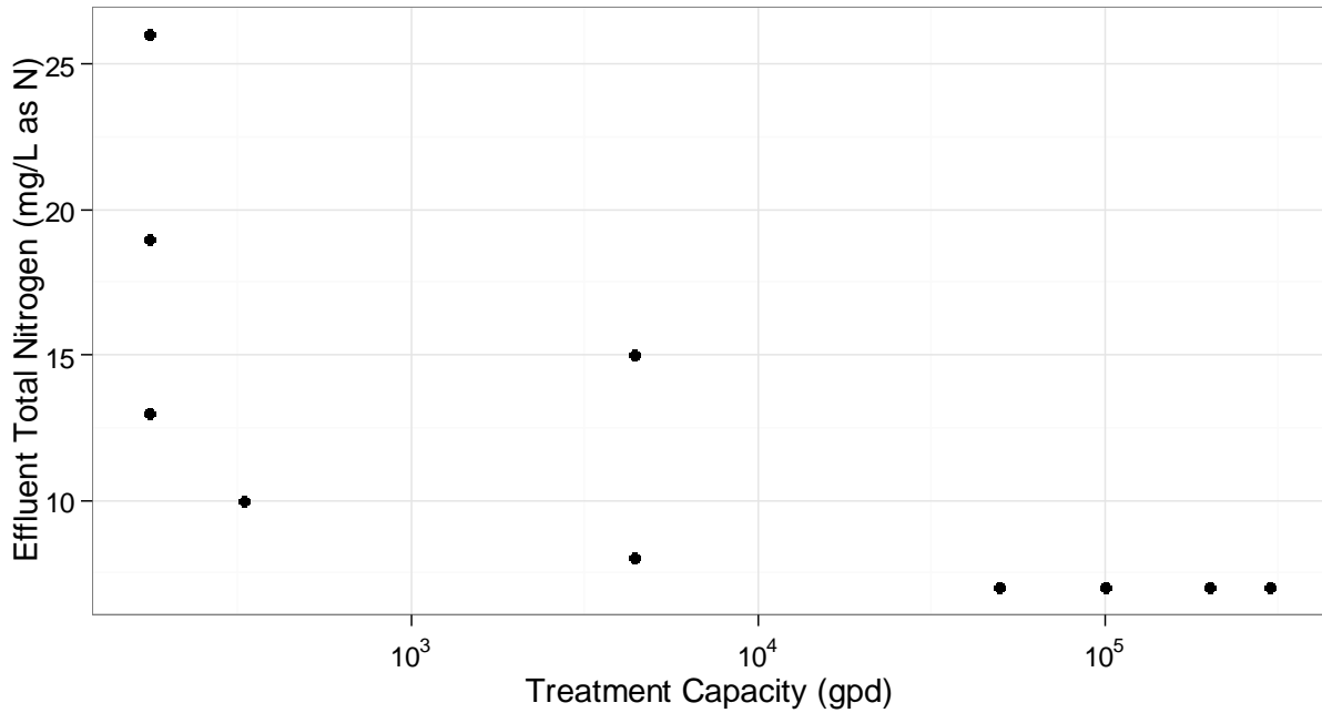
Figure IV-19. TN effluent quality and decentralized treatment system capacity.
